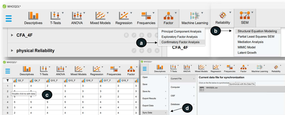
Figure 1: Key Modules for CFA, Visualization, and Data Synchronization in JASP
